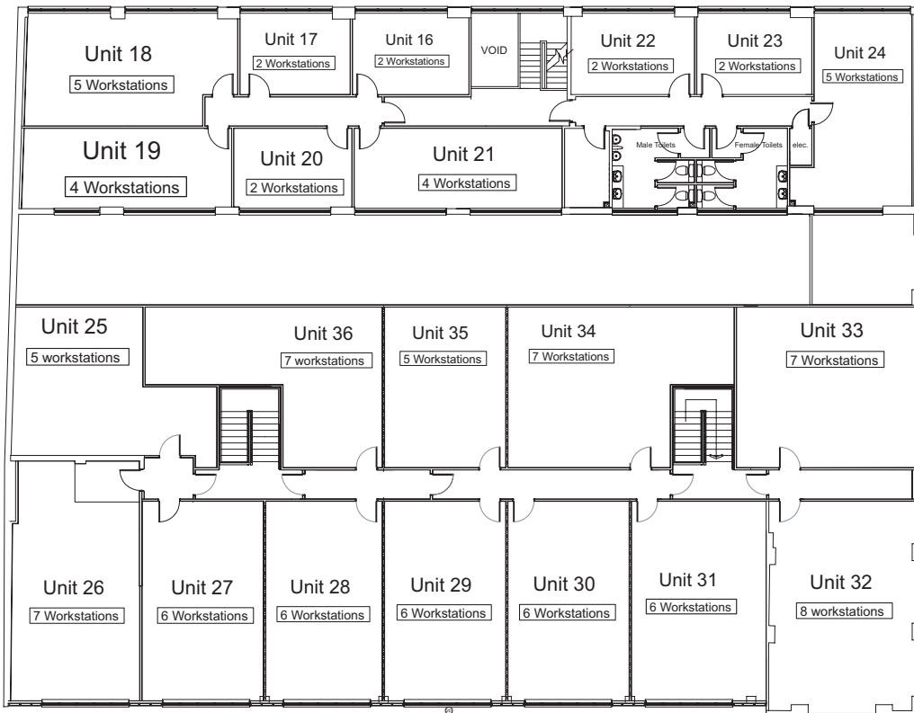
FIRST FLOOR
